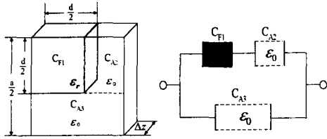
Fig. 4 A Synthesized Capacitance Model.
