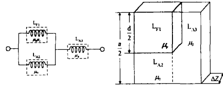
Fig. 5 A Synthesized Inductance Model.
