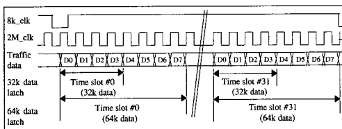
Fig. 3 Traffic data latch timing from trunk
