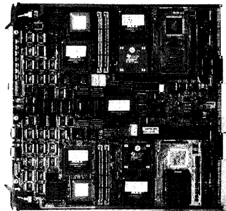
Fig. 12 Implemented Modulator channel card
