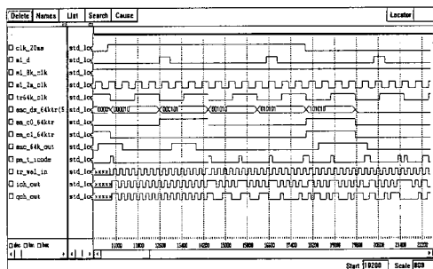
Fig. 6 Timing simulation of channel coding & spreading module of Traffic channel
