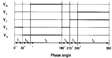
(b) Three buffer type
