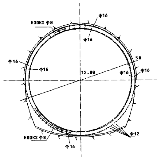
Fig. 4. Typical section of the reinforced concrete lining of Bakun diversion tunnel ∴ φ16: 주철근 BSB460 철근지름 16 mm HOOKS φ8: 간격유지철근 BSB460 철근지름 8 mm
