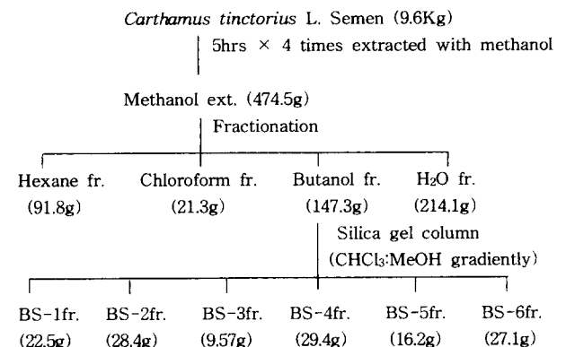
Scheme 1. Fractionation of Carthamus tinctorius L. Semen
