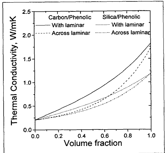
Fig. 9. Predicted thermal conductivities of carbon/phenolic and silica/phenolic composites with varying the volume fraction of fiber at RT
