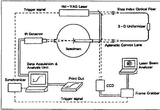
Fig. 1. Schematic diagram of laser flash equipment
