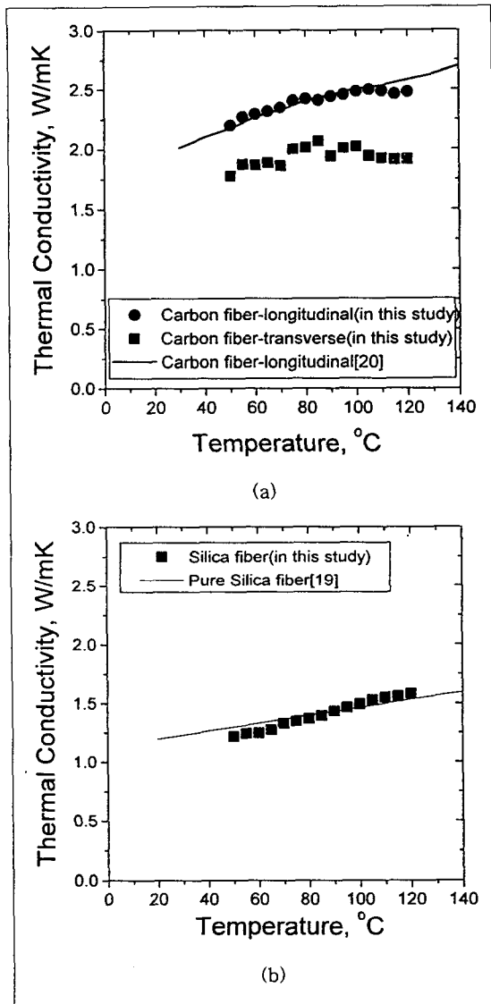
Fig. 8. Calculated thermal conductivities of fibers from thermal conductivities of carbon/phenolic and silica/phenolic composites with varying temperature. (a) carbon fiber and (b) silica fiber
