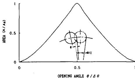
Fig. 3 Area Change for Rotary Valve
