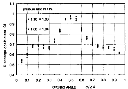
Fig. 4 Variation of Discharge Coefficients with Valve Opening Angle
