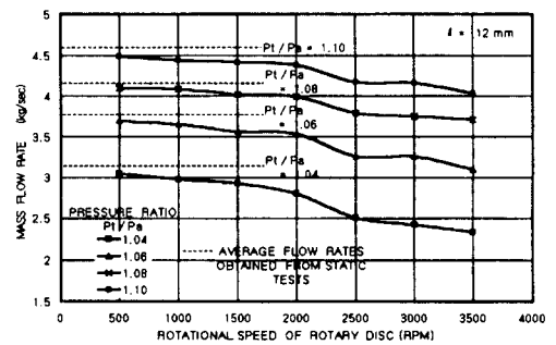
(b) disk thickness 12mm
