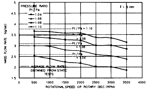
(a) disk thickness 6mm
