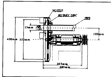
(b) Rotary Valve Assembly
