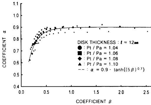
Fig. 7 Variation of Coefficient \alpha with \beta
