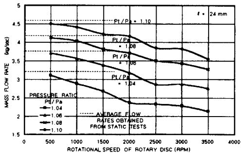
Fig. 5 Comparison of Mass Flow Rate with Rotational Speed
