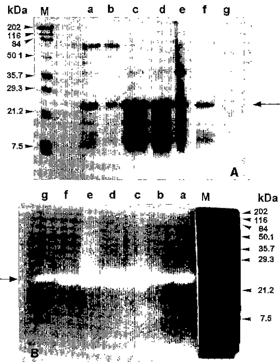
Fig. 1. Cell wall lytic enzyme pattern of total soluble protein in extracellular and intracellular extract of Penicillium oxalicum (HCLF-34). A, SDS-PAGE; B, renaturation SDS-PAGE. Lane M, molecular weight maker; a, cut off extracellular enzyme by 300 kDa ultrafiltration membrane; b, 100 kDa; c, 50 kDa; d, 30 kDa; e, 10 kDa; f, 3 kDa; g, intracellular enzyme.
