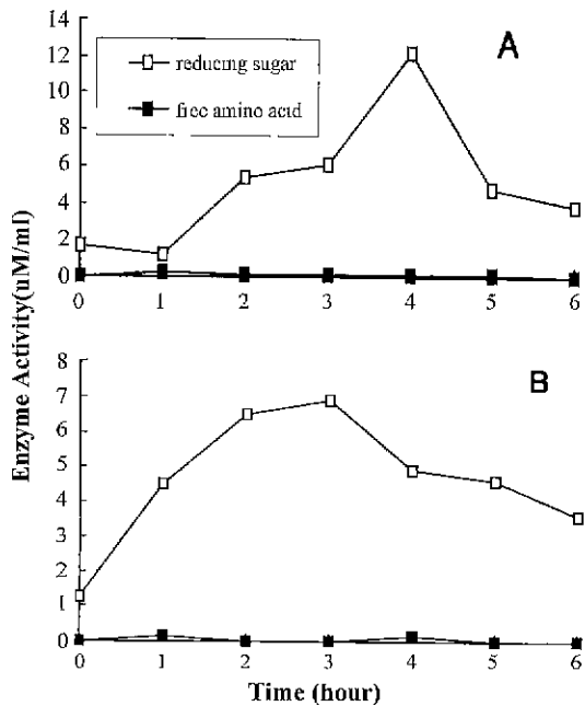
Fig. 3. Activities of extracellular enzyme from Penicillium oxalicum (HCLF-34) against cell wall extracts from Anabaena cylindrica (A) and Micrococcus luteus (B).
