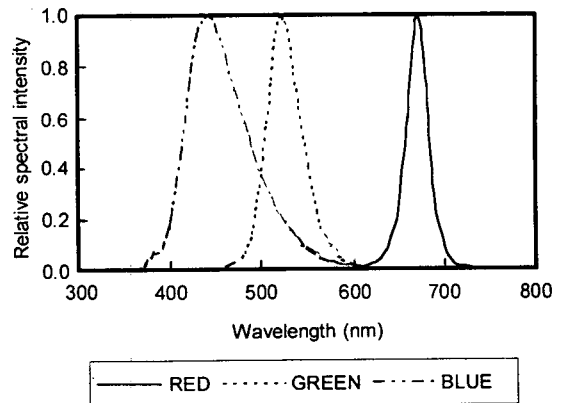
Fig. 3 Relative spectral intensity of blue, green, and red LEDs.
