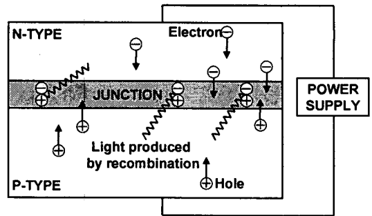
Fig. 1 Principle of light emitting in LEDs.
