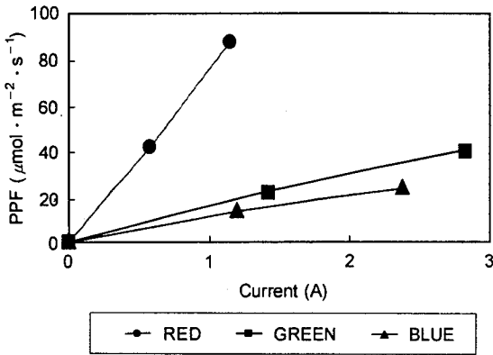
Fig. 7 Relation between PPF of blue, green, red LEDs and the applied current.
