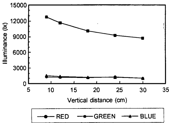
Fig. 5 Variation of illuminance affected by the vertical distance from LEDs.
