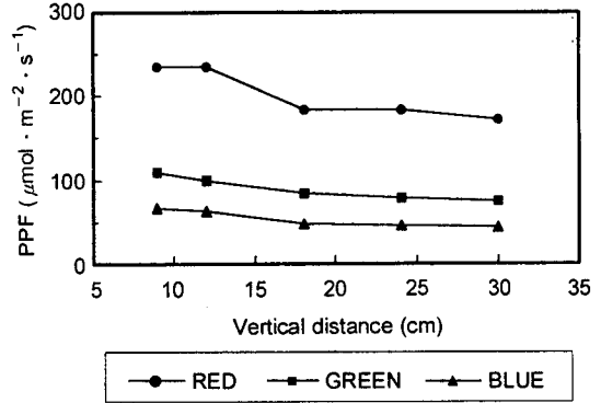
Fig. 4 Variation of photosynthetic photon flux (PPF) affected by the vertical distance from LEDs.
