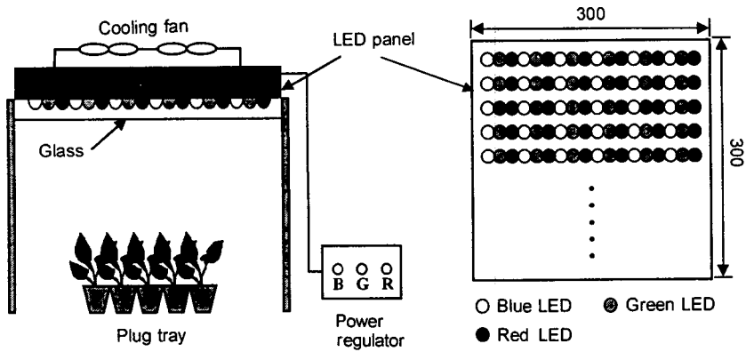
Fig. 2 Schematic diagram of LED module and power regulator.
