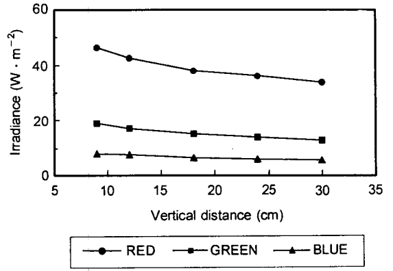
Fig. 6 Variation of irradiance affected by the vertical distance from LEDs.
