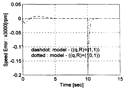
(b) speed error response
