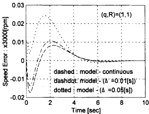
(b) speed error response
