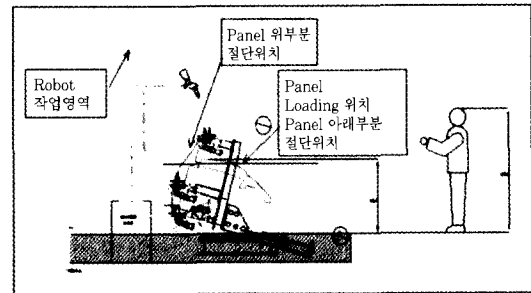
Fig. 5 Jig layout of laser cutting system
