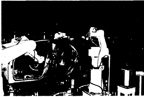
Fig. 4 Photo of In Line Measuring System
