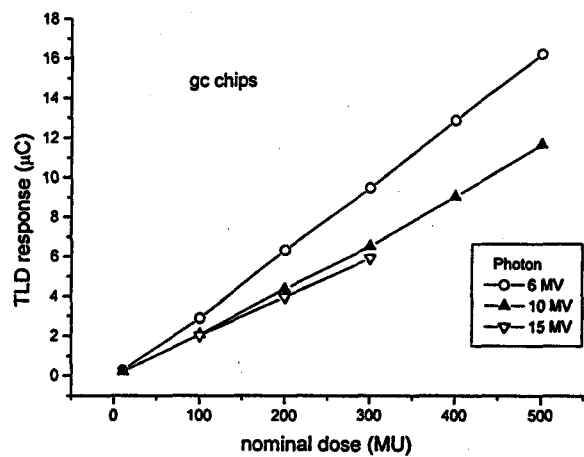
Fig. 3. Relative surface dose response curves for TLD with Gold plate. Each curve is for one photon energy.
