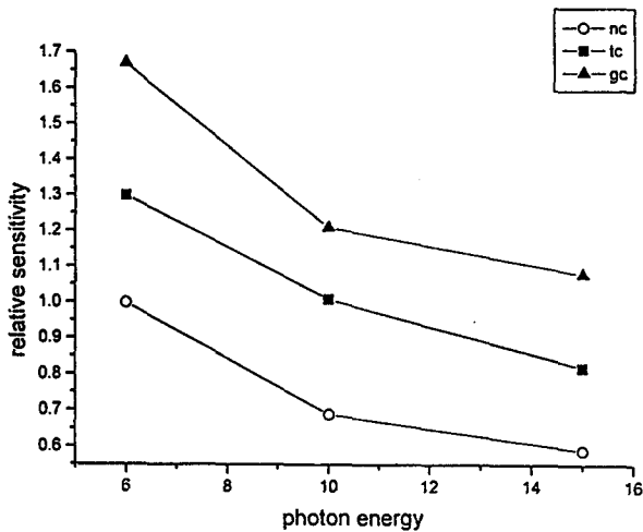
Fig. 4. Energy dependence plotted as photon beam energy against relative sensitivity to normal TLD.
