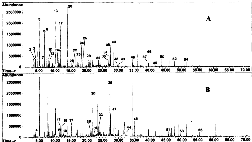
Fig. 3. Total ion chromatogram for the flavor compounds of propolis by GC/MS.; A: falseacacia, B: chestnut tree
