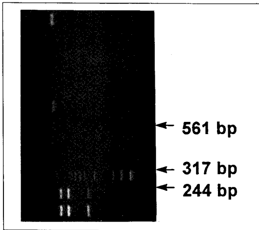
Fig. 1. Agarose gel electrophoresis of pncA gene after BstB I digestion. The PCR product is 561 bp fragment. After incomplete digestion, 561, 317, and 244 bp fragments were seen.
