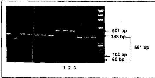
Fig. 3. Agarose gel electrophoresis of pncA gene of M. tuberculosis and M. bovis after BstE II digestion.
