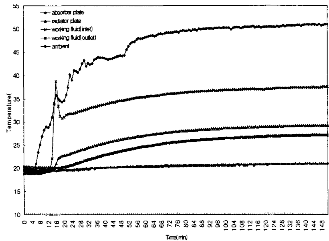
Fig. 9. Laboratory test results for the Loop-type thermo-diode
