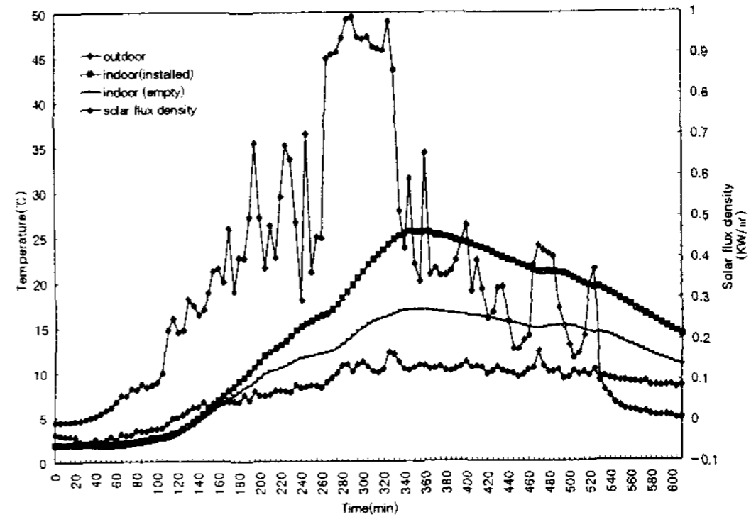
Fig. 11. Indoor temperature comparison of two test cell (with and without Smart Module)
