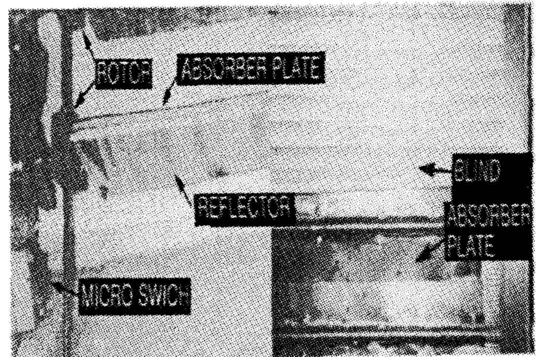
Fig. 7. Absorber design of the Loop type thermo-diode a. rotation type(left), b. blind type(right)
