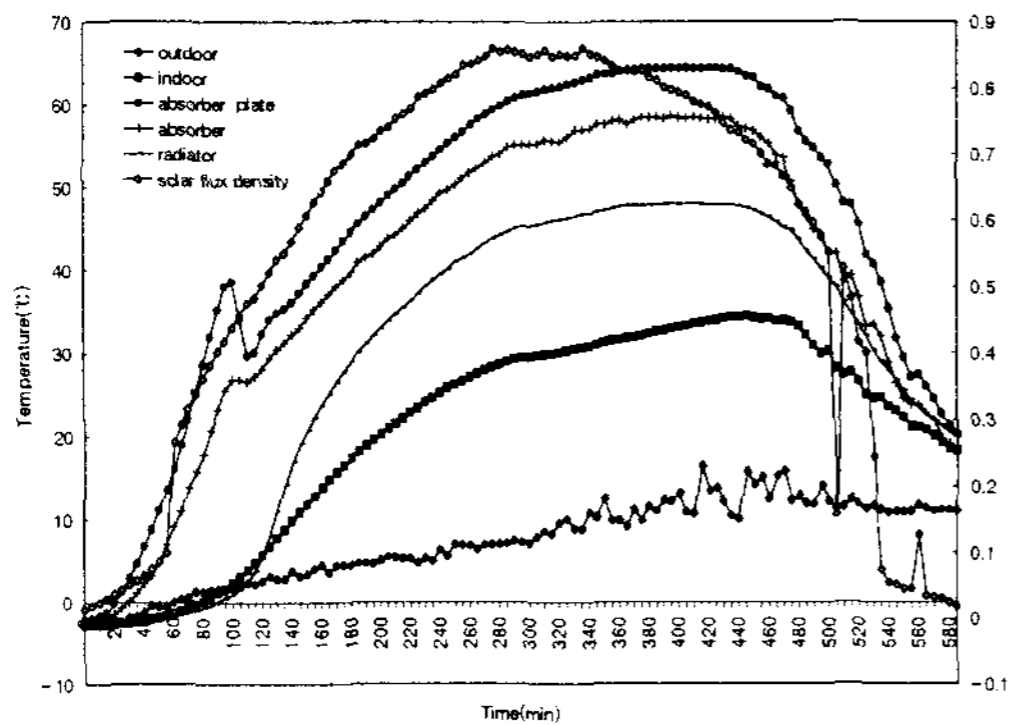
Fig. 10. Result of the outdoor test for the thermo-diode
