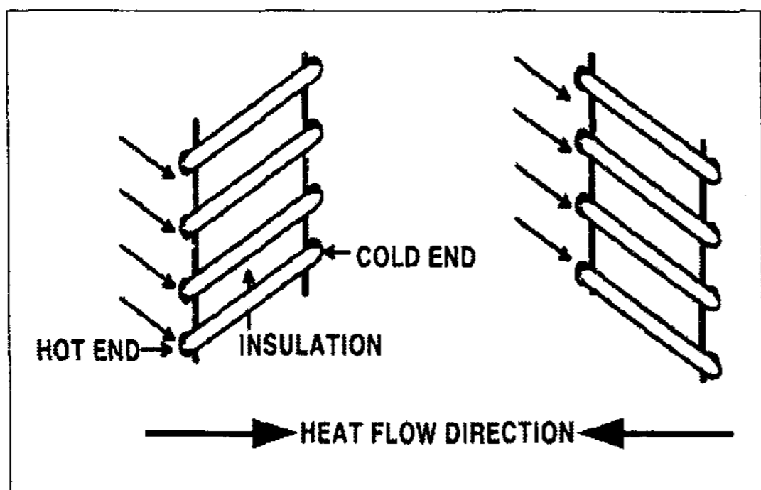
Fig. 5. A bidirectional rectangular thermo-diode design
