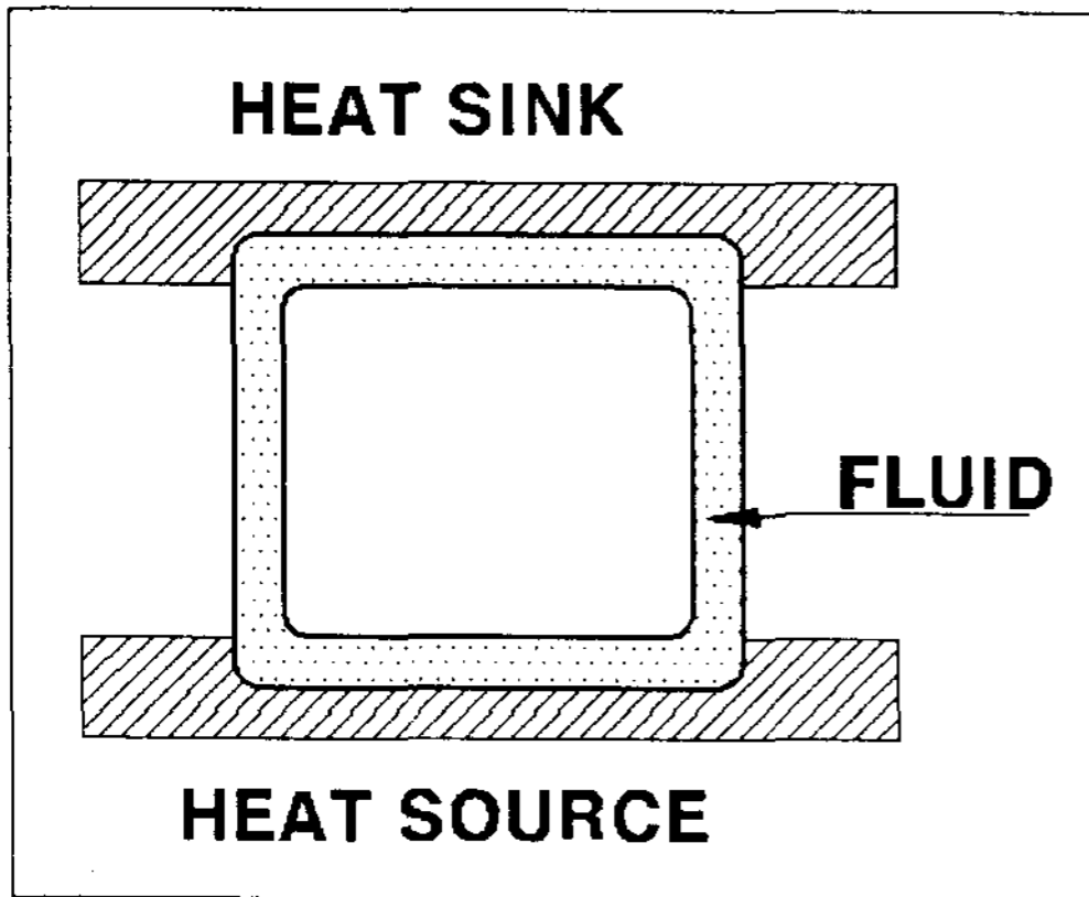
Fig. 2. A rectangular closed-loop thermo-diode
