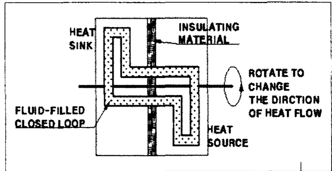
Fig. 3. Bidirectional thermo-diode
