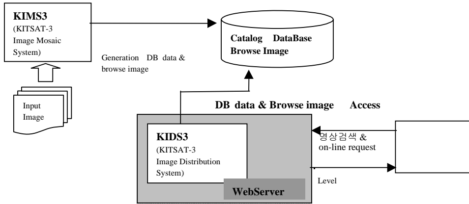
FIGURE 1. KIDS3 operation flow
