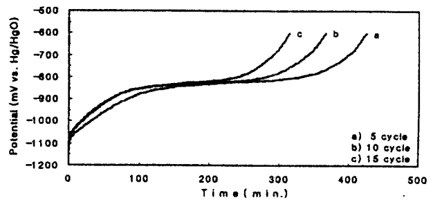
Fig. 11. Discharge curves of sintered Ti_{0.85}FeMn_{0.15} electrode at 10wt.% Ni electroless plating(discharge rate 10mA/g)
