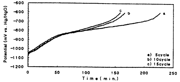
Fig. 10. Discharge curves of sintered TiFe electrode at 10wt.% Ni electroless plating(discharge rate 10mA/g)
