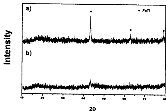
Fig. 2. X-ray diffraction pattering of FeTi powders
