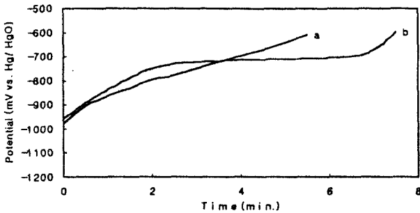
Fig. 5. Discharge curves of FeTi electrodes prepared with a) non-treated powder and b) Ni electroless plated powder(discharge rate : 10mA/g)
