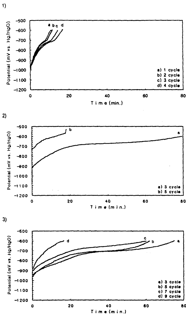
Fig. 6. Discharge curves of FeTi electrodes using powders heat-treated at 1)400°C, 2) 800°C and 3) 1000°C before shaping(discharge rate : 10mA/g)
