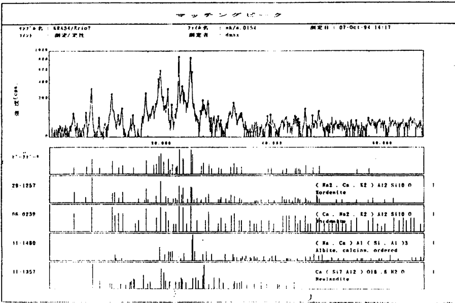
Fig. 8. Youngil zeolite mineral contaminated mordenite and clinoptilolite by XRD.
