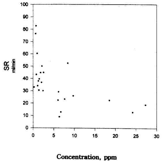
Fig. 3. Sampling rate of korean passive sampler for trichloroethylene by concentration.
