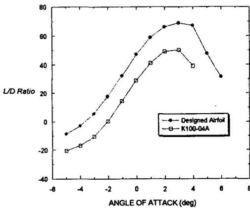
(b) L/D Ratio
