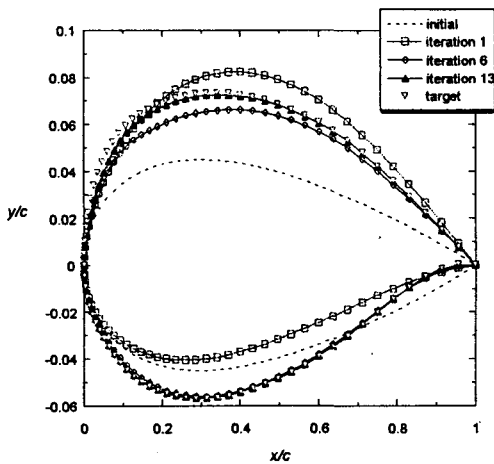
(a) Airfoil geometry
