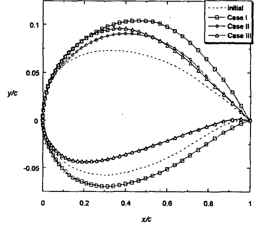
(a) Airfoil geometries
