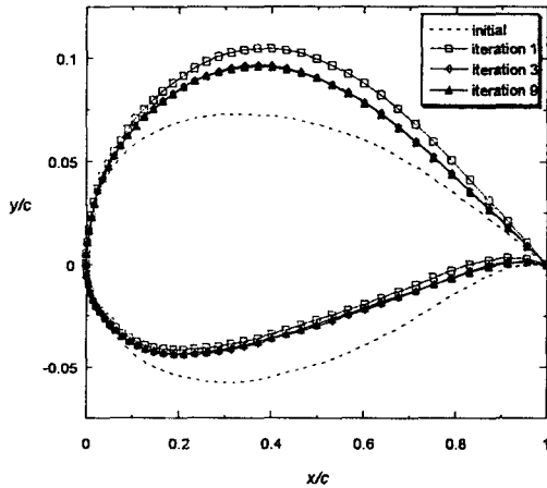
(a) Airfoil geometry
