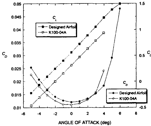
(a) C_L and C_D
