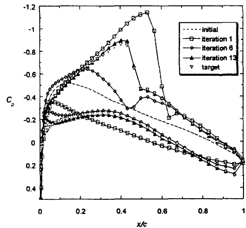
(b) Surface pressure distribution
