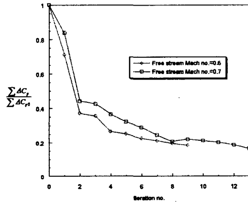
Fig. 3 Convergence histories of testcase I.
