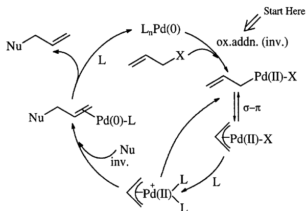
Figure 1. The general reaction mechanism of the Pd(0)-catalyzed reaction of allylic compounds.
