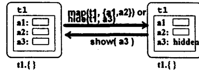
Figure 13: The attribute operations
