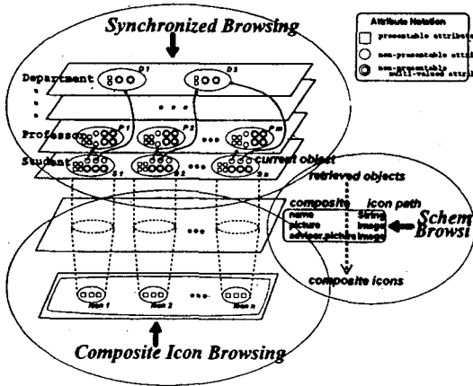
Figure 2: Browsing Techniques and Object of COMIB
