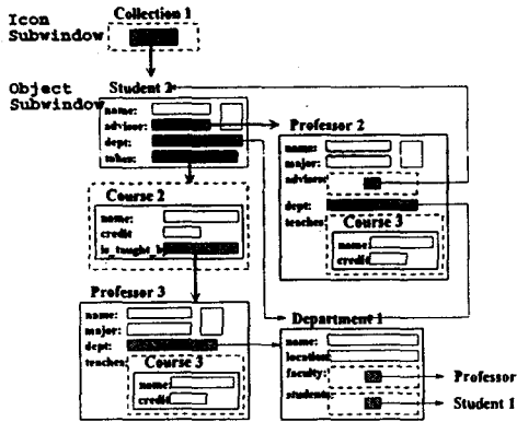
Figure 10: Transformed presentation information objects
