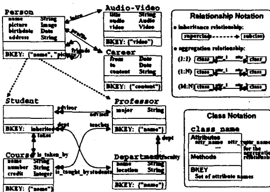
Figure 1: University Schema
