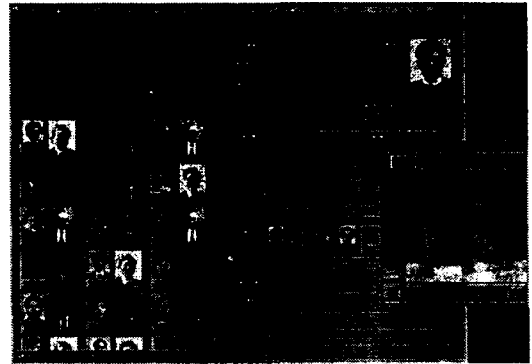
Figure 7: synchronized browsing
