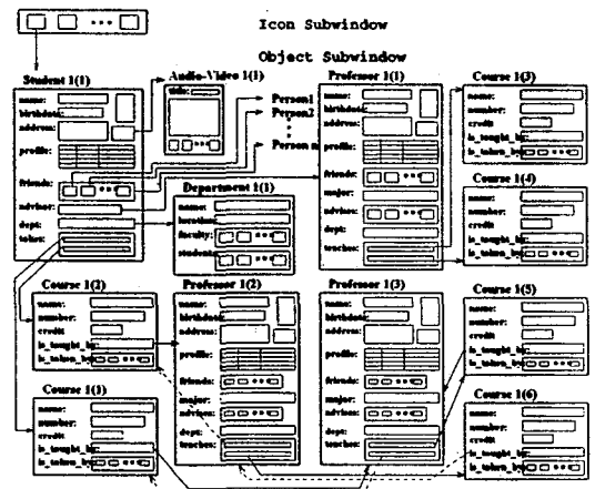
Figure 9: Browsing a Student object according to the default presentation information objects
