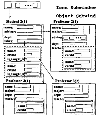
Figure 11: Browsing the customized view of a Student object
