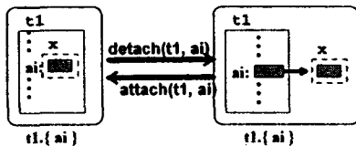
Figure 12: The form operations
