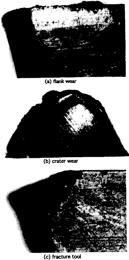
Fig. 2 Shape of tool (a) flank wear, (b) crater wear, (c) fracture tool
