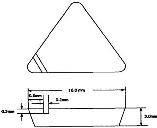
Fig. 1 Dimensions of slotted insert
