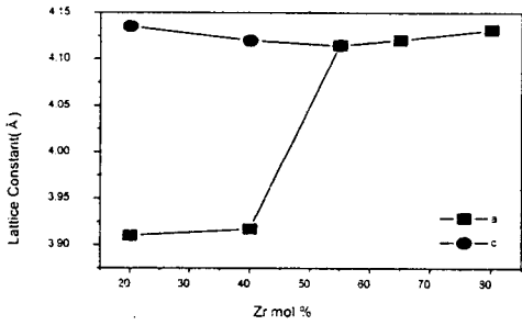
(a) Variation of lattice constant with Zr mol %
