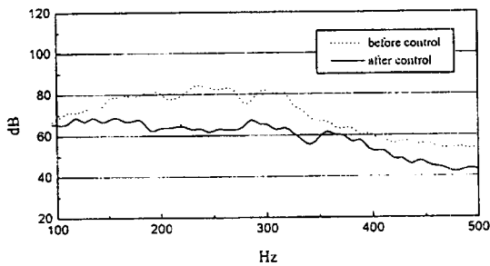
(b) Constrained Filtered-X LMS algorithm
