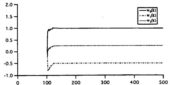
(b) Coefficients adjustment versus iteration number
