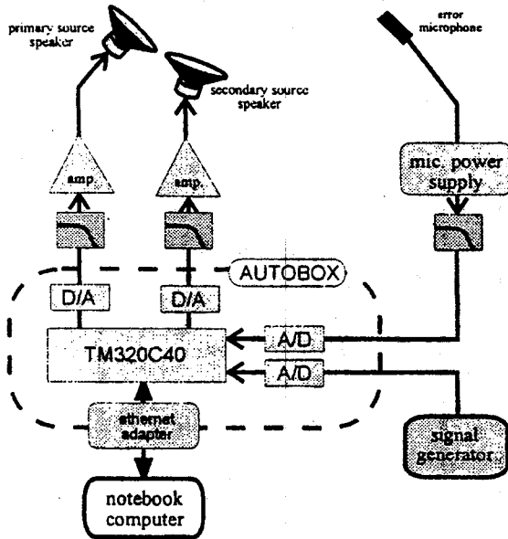
Fig. 5 Experimental setup
