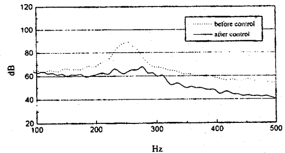
(b) Constrained Filtered-X LMS algorithm
