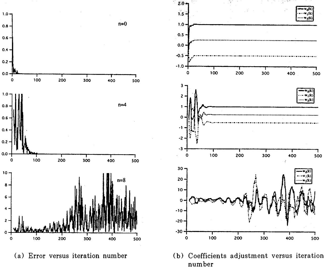
Fig. 3 Learning curves in case of the filtered-x LMS algorithm( q=2; \eta=0.5; n=0,4,8 )
