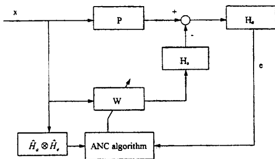
Fig. 2 Block diagram of the active noise control system with an adaptive FIR filter
