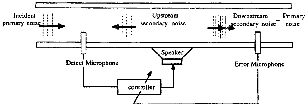
Fig. 1 Schematic diagram of the active noise control process in duct
