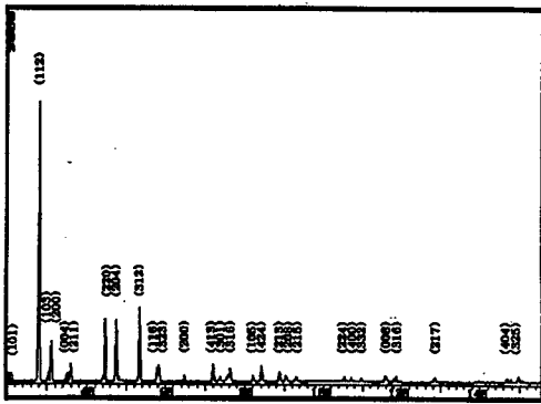
Fig. 3. X-ray diffraction patterns of AgGaS 2 polycrystal.
