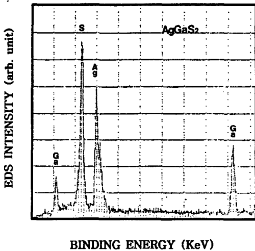
Fig. 5. EDS of AgGaS 2 single crystal thin films.
