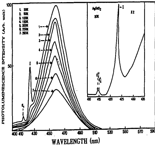
Fig. 10. Photoluminescence spectra of AgGaS 2 single crystal thin films.
