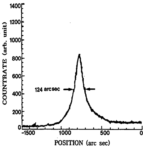
Fig. 4. Double crystal X-ray rocking curve of AgGaS 2 single crystal thin films measured growth temperature of substrate of 440°C.
