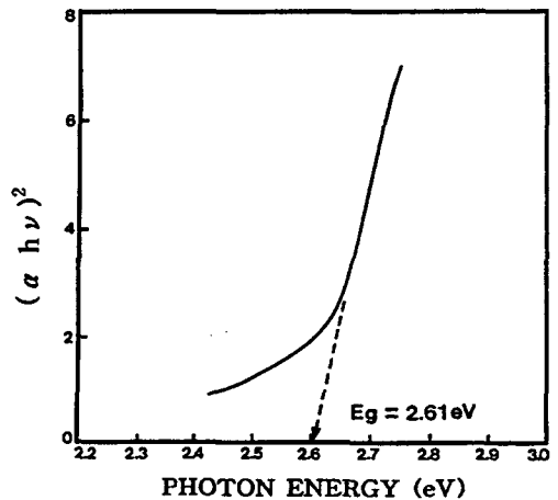
Fig. 7. Plots (\alpha h\nu)^2 versus the incident photon energy h\nu for AgGaS 2 single crystal thin films
