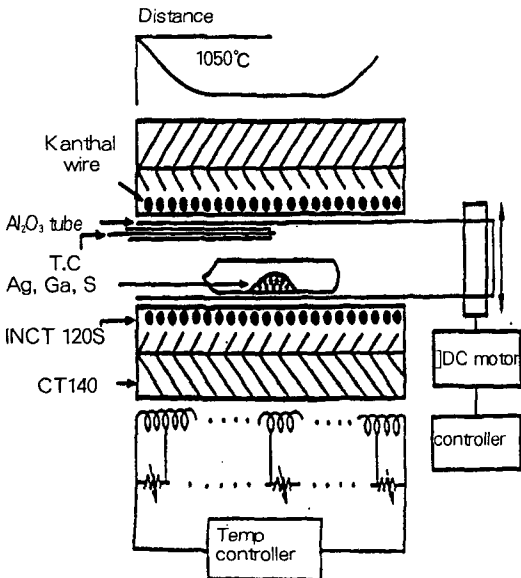
Fig. 1. Horizontal furnace for synthesizing of AgGaS 2 polycrystal.
