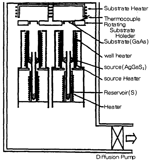
Fig. 2. Block diagram of the hot wall epitaxy system.
