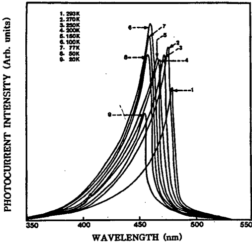
Fig. 8. Photocurrent spectra of AgGaS 2 single crystal thin films.
