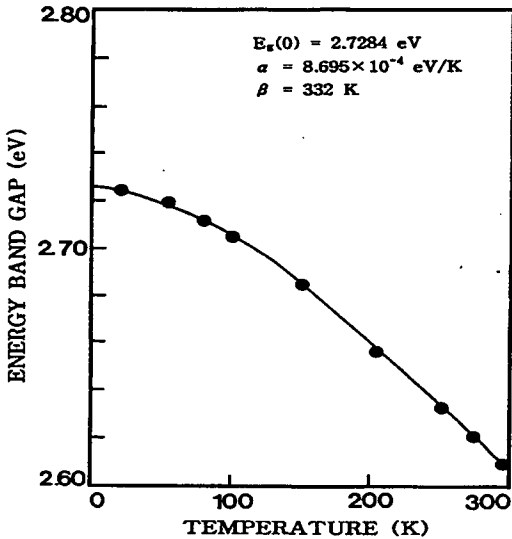
Fig. 9. Temperature dependence of the energy gap in AgGaS 2 single crystal thin films (The solid line represents the fit to the Varshni equation).
