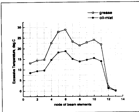
Fig. 5 Beam elements excessive temperature on the lubricant type
