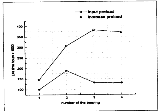
Fig. 8 Bearing life time on the preload
