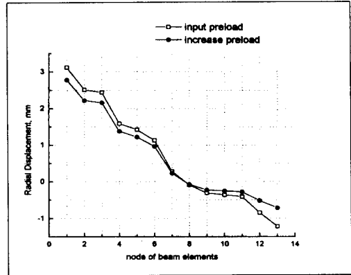
Fig. 7 Flexible line of spindle on the preload
