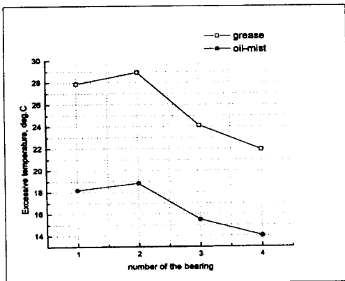
Fig. 6 Bearing excessive temperature on the lubricant type
