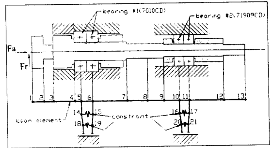
Fig. 1 Modeling of the spindle
