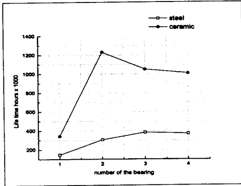
Fig. 4 Bearing life time on the ball material
