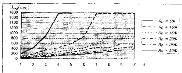
(a) k=4
