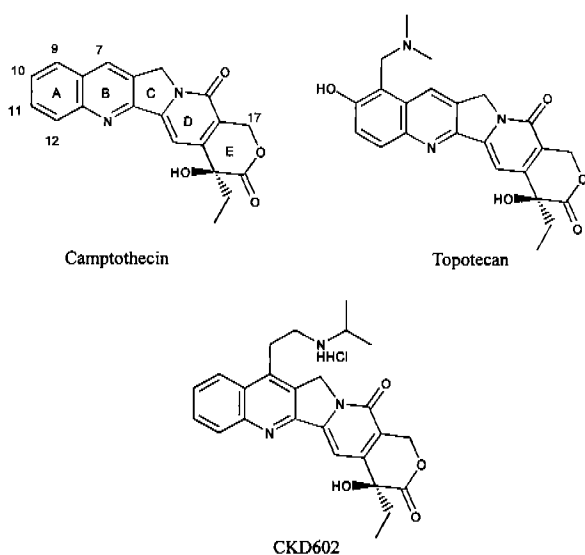
Fig. 1. Chemical structures of CKD602, topotecan, and camptothecin.
