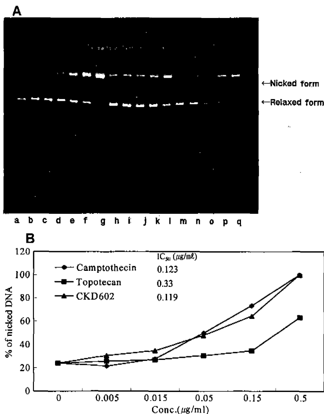
Fig. 2. Comparison of topoisomerase I-mediated DNA cleavage induced by camptothecin, topotecan, and CKD602. Supercoiled pBR 322 (0.25 µg) was incubated with 4 units of human topoisomerase I in the presence or absence of drugs followed by SDS/proteinase K treatment and then analyzed on an agarose gel containing 0.5 µg/ml EtBr. Lane a, substrate pBR 322; b, no drug; c~g, camptothecin; h~l, topotecan; m~q, CKD 602. Drug concentrations were: lane c, h, and m, 0.005 µg/ml; d, i, and n, 0.015 µg/ml; e, j, and o, 0.05 µg/ml; f, k, and p, 0.15 µg/ml; g, l, and q, 0.5 µg/ml.
