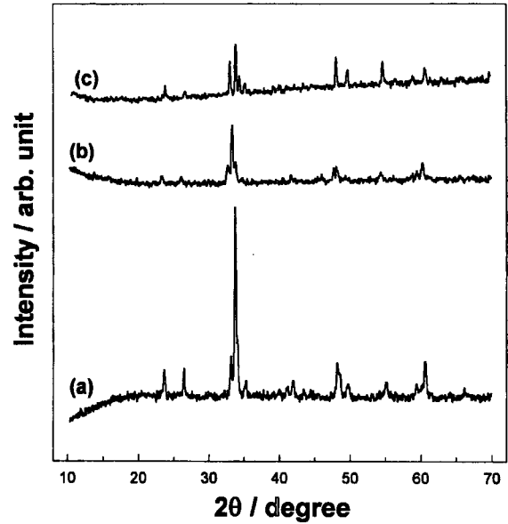
Fig. 4. X-ray diffraction patterns of Gd_{0.5}Ca_{0.2}Co_{0.7}Fe_{0.3}O_3 . (a) as-prepared, (b) after a heat-treatment at 1300^\circ C for 1.5 h, and (c) after a heat-treatment at 1400^\circ C for 1.5 h. Note that this material is thermally stable up to 1400^\circ C .
