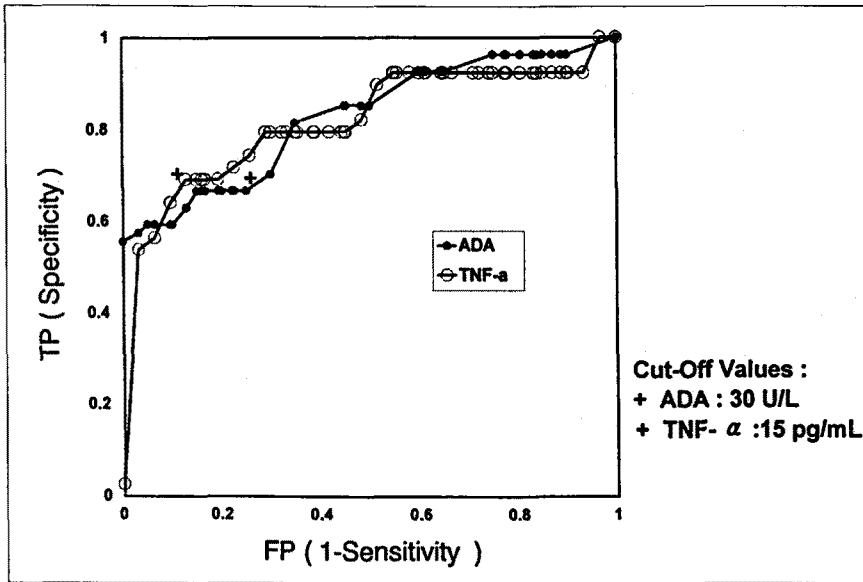
Fig. 3. Receiver operation characteristics curve for adenosine deaminase(ADA) and tumor necrosis factor(TNF- \alpha )
