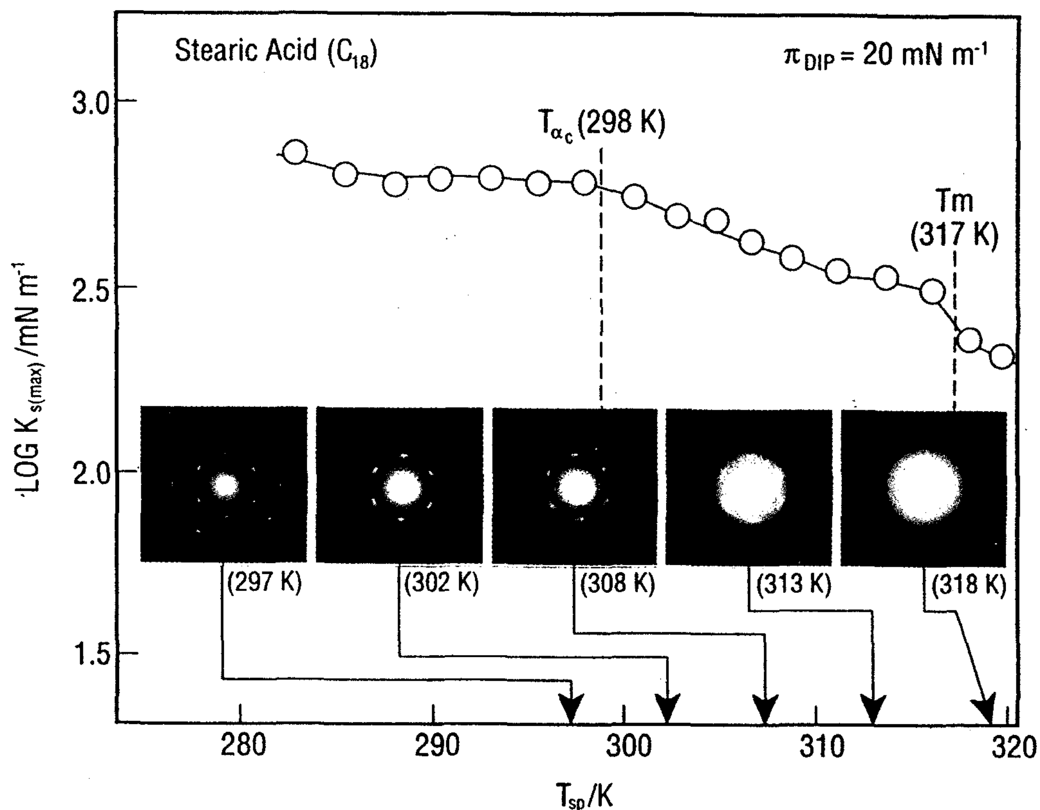
Figure 2. T_{sp} dependence of \log K_{s(\text{max})} , and electron-diffraction patterns of stearic-acid monolayers.
