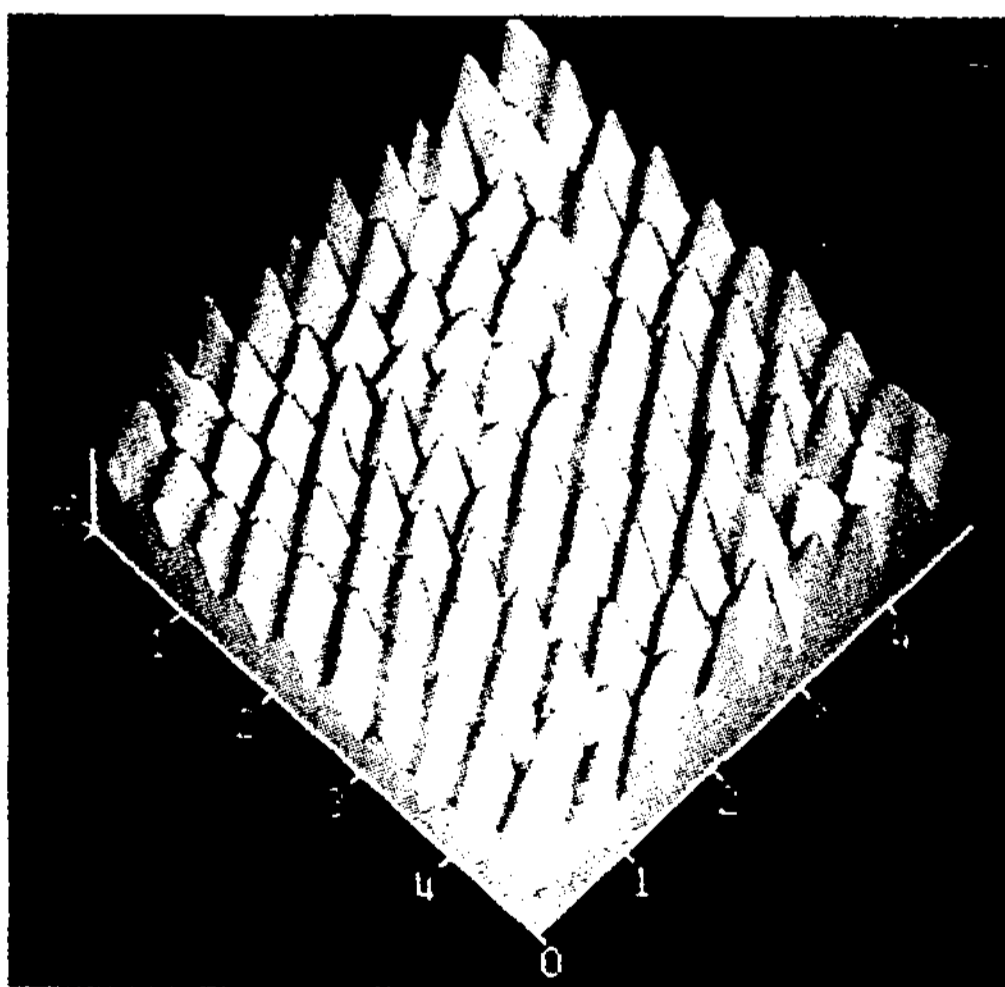
Figure 8. Filtered AFM image of a stearic-acid monolayer on a scan area of 5 \times 5 \text{ nm}^2 . The stearic-acid molecules were regularly arranged in a hexagonal array with a (10) spacing of 0.42 nm.
