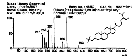
Fig. 5. Electron impact mass spectrum and library spectrum of Clc.
