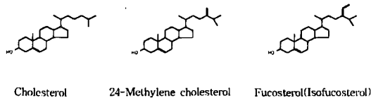
Fig. 7. Structures of compound I.
