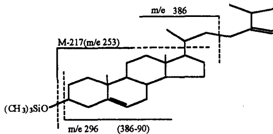
Fig. 6. Mass fragmentation of Clb.
