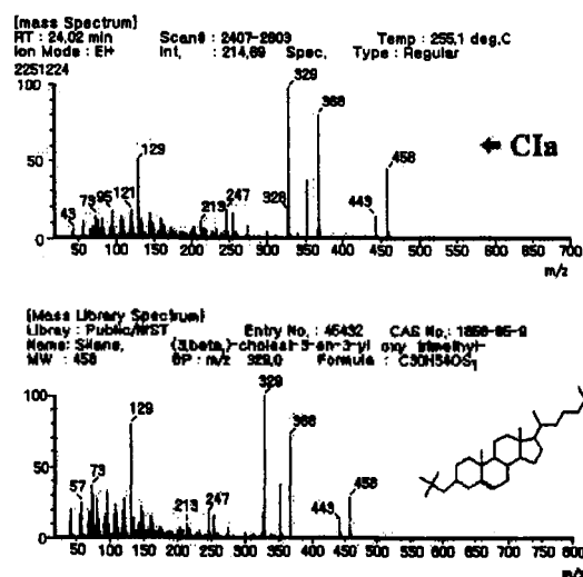
Fig. 3. Electron impact mass spectrum and library spectrum of C1a.
