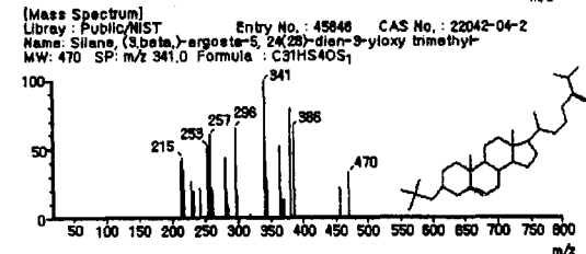
Fig. 4. Electron impact mass spectrum and library spectrum of Clb.
