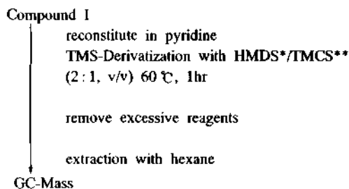
Fig. 1. GC-Mass analysis procedure by compound I derivatization with TMS. (*; Hexamethyldisilazane, **; Trimethylchlorosilane)
