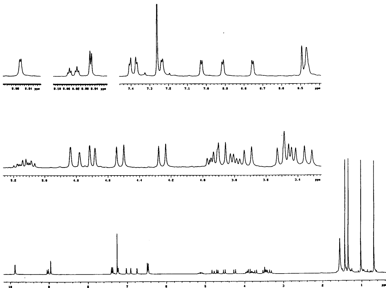
Figure 1. ^1\text{H} NMR spectrum of Chiral Calix[4]arene 4a .
