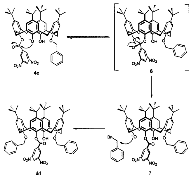
Figure 2. The Proposed Reaction Pathway for 1,2,4-Trisubstitution.
