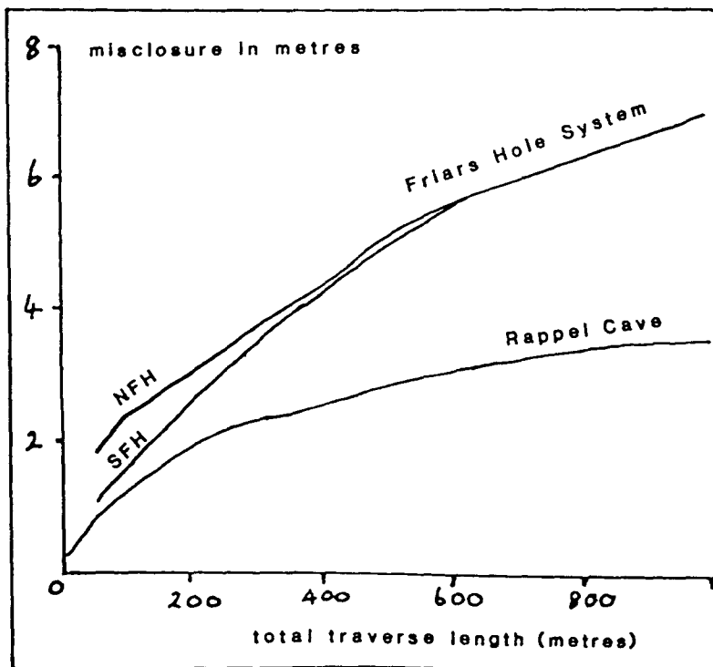
Figure 1. Misclosure plotted against.
