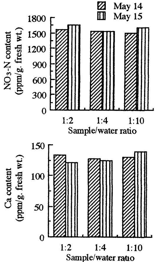
Fig. 3. Relationship between mineral element content in petiole(1 to 20th node) sap and sample/water rate for extraction.
