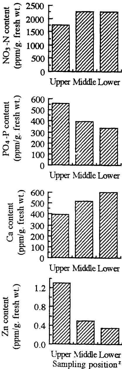
Fig. 6. Effect of sampling position of petioles on mineral element content of the sap.
