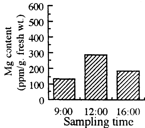
Fig. 5. Effect of sampling time on mineral element content in petiole(1 to 20th node) sap.
