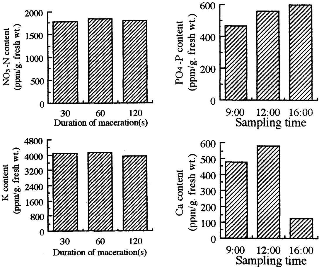
Fig. 4. Relationship between mineral element content in petiole(1 to 20th node) sap and duration of maceration.
