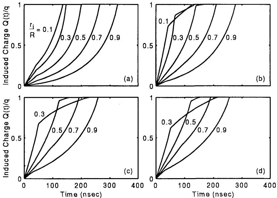
Fig. 5. The Induced Signal Shapes for Various Initial Positions of a Charge Carrier Pair. The Initial Axial Positions ( z_i/L ) are 0.1 (a), 0.3 (b), 0.5 (c) and 0.7 (d), Respectively. The Initial Radial Positions ( r_i/R ) are Indicated by the Lines.
