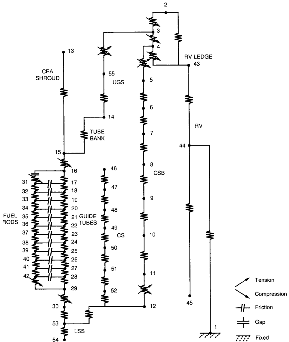
Fig. 2. Lumped Mass Model of Coupled Internals and Core in the Vertical Direction
