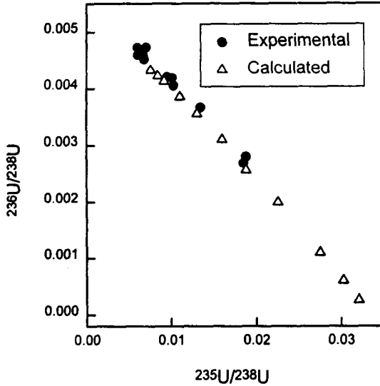
Fig. 2. Correlation Between ^{236}\text{U}/^{238}\text{U} and ^{235}\text{U}/^{238}\text{U} Atom Ratio
