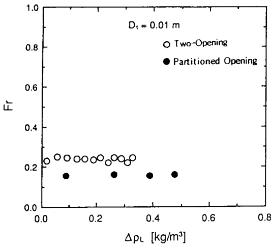
Fig. 9. Variation of Froude Number with Density Increment
