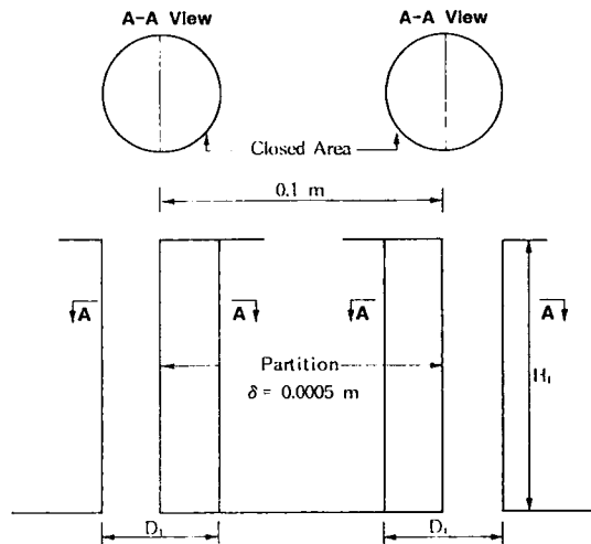
Fig. 5. Schematic Diagram of Two-Opening
