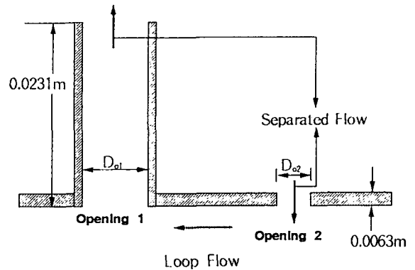
Fig. 12. Schematic Diagram of Loop Flow Observed by Epstein in Two-Opening System[2]
