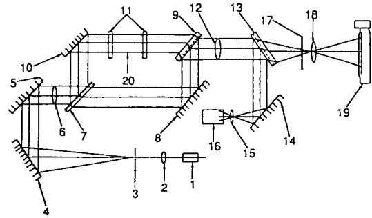
Fig. 6. Optical Components of Mach-Zehnder Interferometer
