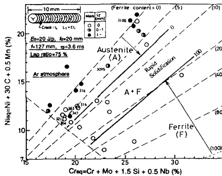
Fig. 3 Crack lengths for various stainless steels subjected to laser-overlapped welding show in the Schaeffer diagram.
