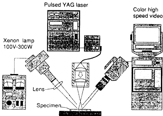
Fig. 1 Schematic arrangement of high speed video photography for observation of fusion and solidification phenomenon occurring laser spot welding.
