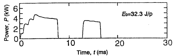
Fig. 11 Output power shape of pulsed YAG laser controlled for reducing cracking, showing second pulse after main laser shot.
