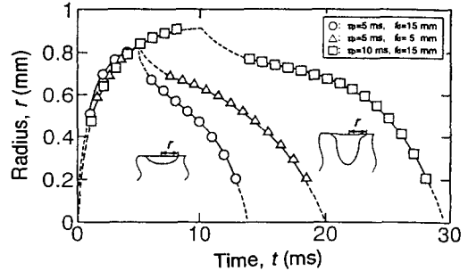
Fig. 9 Variation in radius of laser weld molten puddle of Type 310S as function of time.
