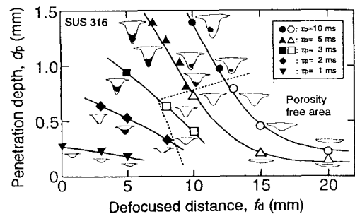
Fig. 4 Effect of penetration depths of weld metals, defocused distance and pulsed length on porosity formation and location in laser spot weld fusion zones.
