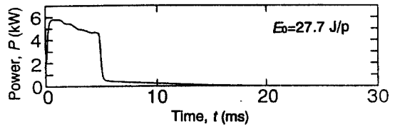
Fig. 10 Output power shape of pulsed YAG laser with tailing of low power, used for heat-conduction mode of spot weld metal.
