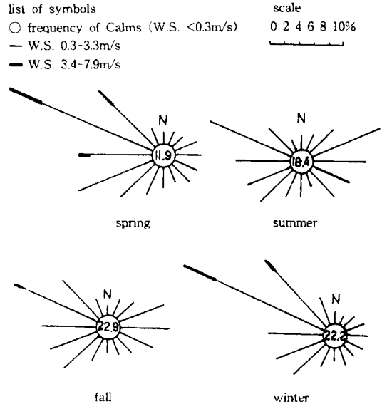
Fig. 4. The seasonal wind rose at Bangi-dong in '96
