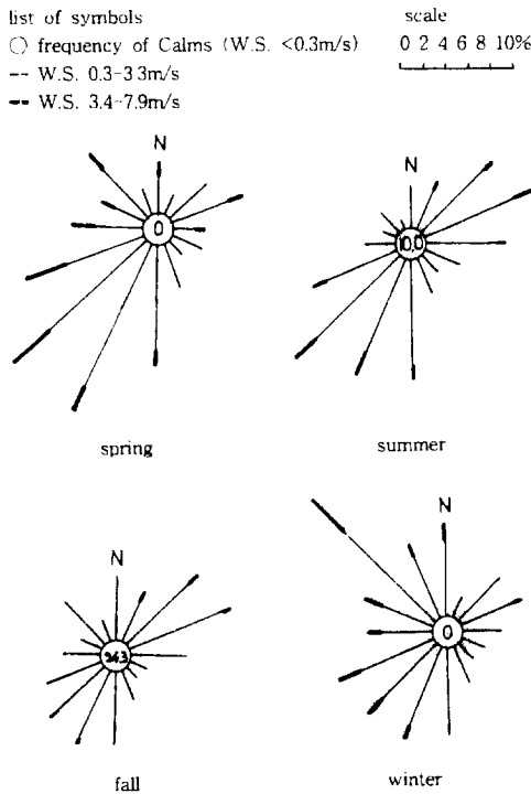
Fig. 3. The seasonal wind rose at Kuro-dong in '96
