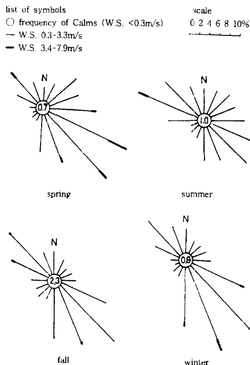
Fig. 1. The seasonal wind rose at Namgajwa-dong in '96
