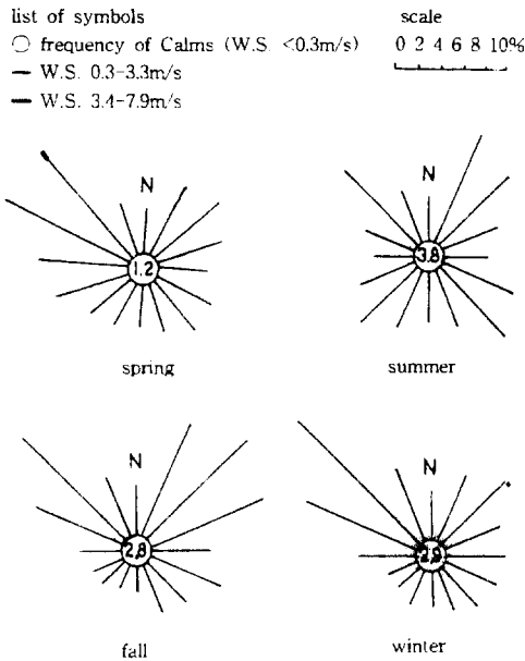
Fig. 2. The seasonal wind rose at Ssangmun-dong in '96
