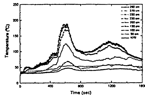
Fig. 4. Temperature profiles on nine elevations of ㉠ position in the fire room for the chair fire.
