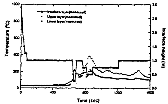
Fig. 15 Average temperature profiles of the upper and lower layer with the change of the interface height for the mattress fire.
