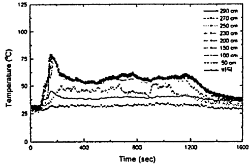
Fig. 5. Temperature profiles on nine elevations of ㉠ position in the fire room for the carpet fire.
