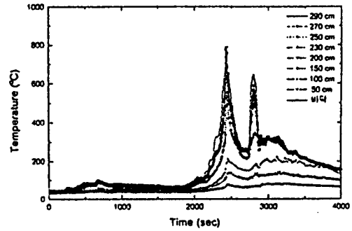
Fig. 8 Temperature profiles on nine elevations of ㉠ position in the fire room for the wardrobe fire.
