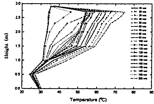
Fig. 9 Average temperature profiles on nine elevations of six positions from 10sec to 200sec for the trashcan fire.
