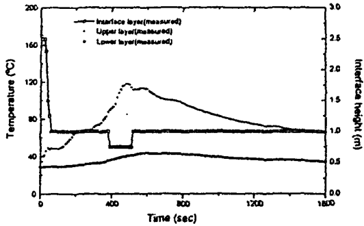
Fig. 11 Average temperature profiles of the upper and lower layer with the change of the interface height for the trashcan fire.
