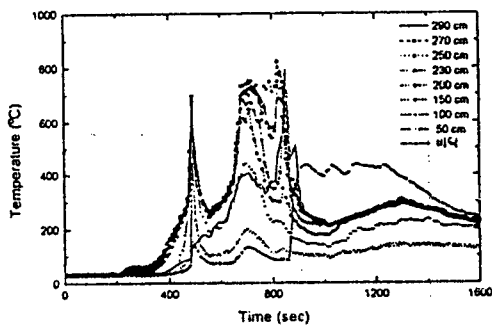
Fig. 6 Temperature profiles on nine elevations of ㉠ position in the fire room for the sofa fire.
