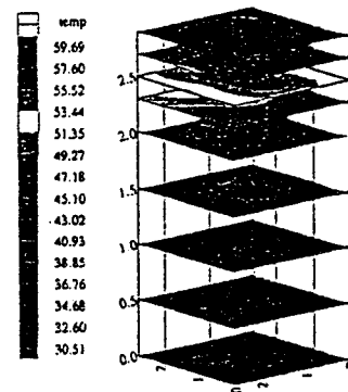
Fig. 10 Temperature distributions on nine elevations at 50sec in the fire room for the trashcan fire.
