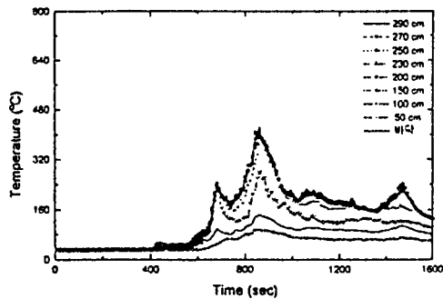
Fig. 7 Temperature profiles on nine elevations of ㉠ position in the fire room for the mattress fire.
