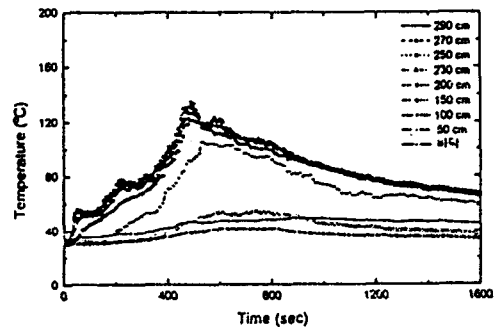
Fig. 3. Temperature profiles on nine elevations of ㉠ position in the fire room for the trashcan fire.
