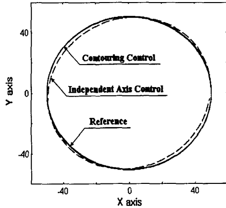
Fig. 10 Circular Contour Response with Mismatched System
