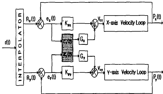
Fig. 3 Structure of an Asymmetrical Contouring Control System
