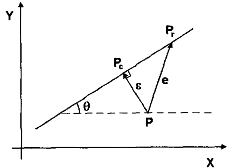
Fig. 2 Tracking and Contouring Error on a Straight Line
