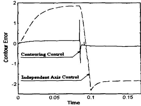
Fig. 9 Contour Error of Corner Path for Independent Axis Control and Contouring Control
