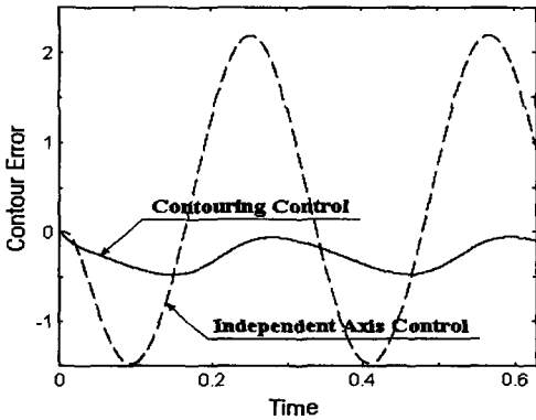
Fig. 11 Contour Error of Circular Path for Independent Axis Control and Contouring Control
