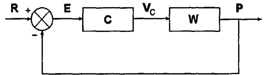
Fig. 4 Block Diagram of the Control Loop
