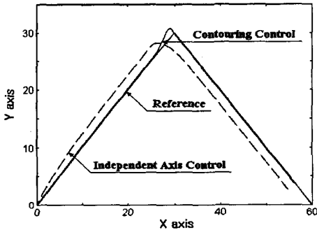
Fig. 8 Corner Contour Response with Mismatched System
