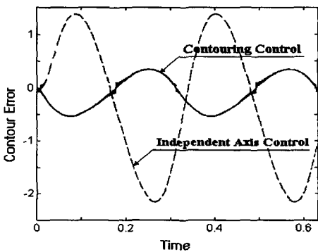
Fig. 13 Contour Error of Elliptic Path for Independent Axis Control and Contouring Control
