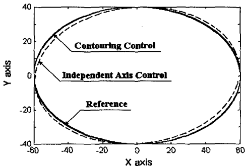
Fig. 12 Elliptic Contour Response with Mismatched System
