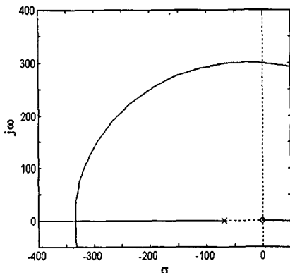
Fig. 5 Root Locus Plot for Contouring Control Gain
