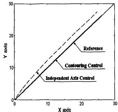
Fig. 6 Straight Line Contour Response with Mismatched System
