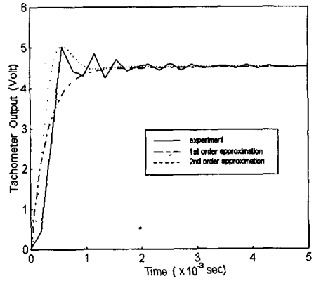
Fig. 1 Experimental Velocity Loop Response to 1 Volt Step Input of V_{ref} and Its Approximated Model Response
