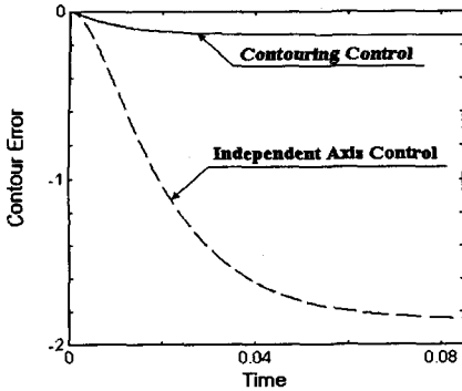
Fig. 7 Contour Error of Straight Line Path for Independent Axis Control and Contouring Control
