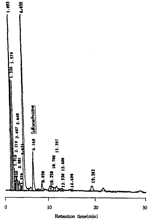
Fig. 2. HPLC chromatogram sulfamethazine fortified milk (50 ppb).
