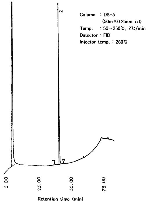
Fig. 2. GC analysis of hexane extract from Agastache rugosa Peak identification (peak 1: eugenol, peak 2: estragole, peak 3: isoeugenol).
