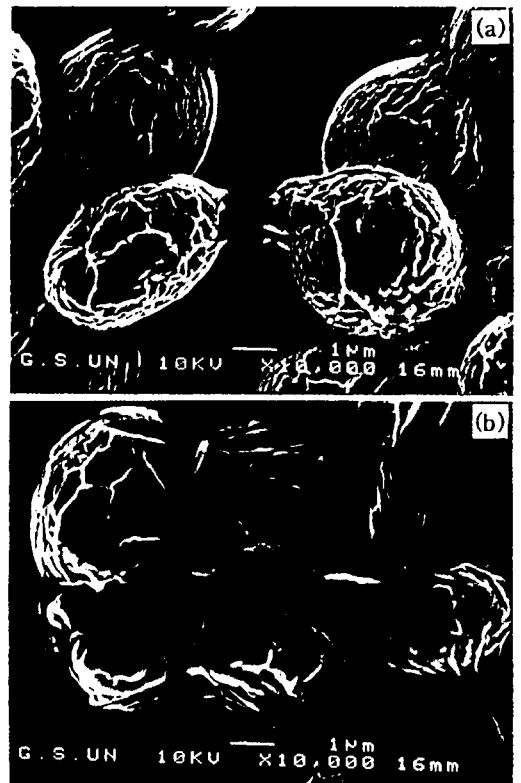
Fig. 9. Scanning electron microscopic view of S. cerevisiae treated with 0.01% estragole. (a: control, b: 0.01% estragole treated).
