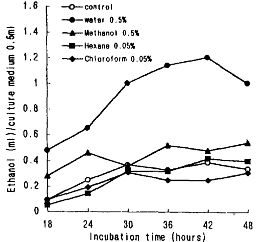
Fig. 7. The effects of extracts and fractions from Agastache rugosa on the unit of ethanol production by S. cerevisiae .
