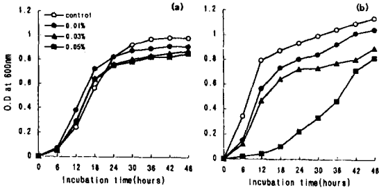
Fig. 5. The growth of S. cerevisiae (a) and S. ellipsoideus (b) in the presence of estragole identified from A. rugosa .
