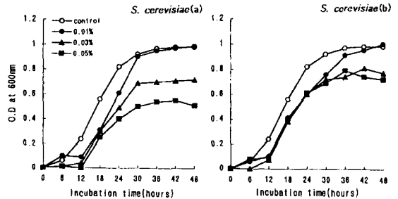
Fig. 4. The growth of S. cerevisiae in the presence of hexane (a) and chloroform fraction (b) from A. rugosa .
