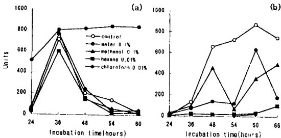
Fig. 8. The effects of extracts and fractions from A. rugosa on the \alpha -amylase (a) by A. oryzae and glucoamylase (b) by A. niger .
