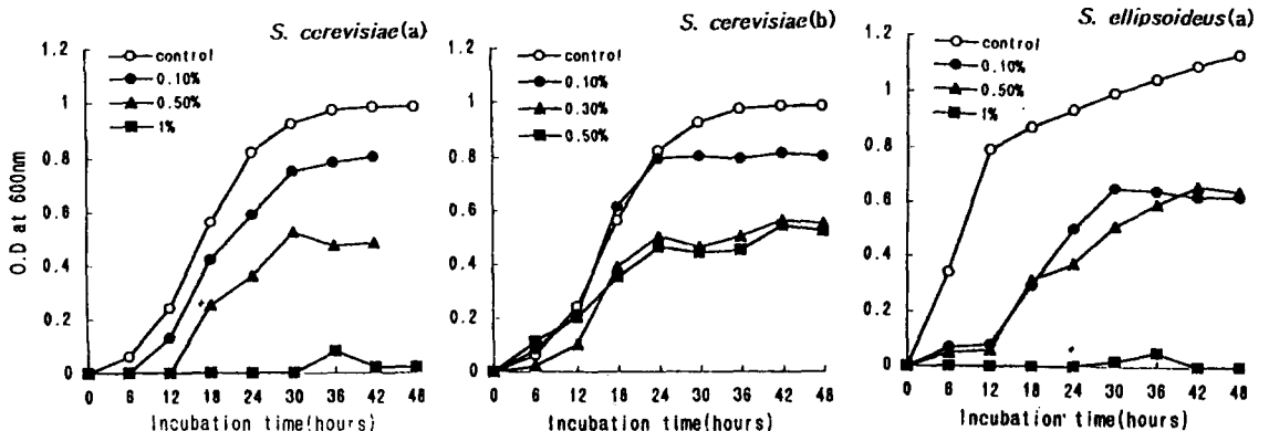
Fig. 3. The growth of S. cerevisiae and S. ellipsoideus in the presence of water (a) and methanol extract (b) from A. rugosa .
