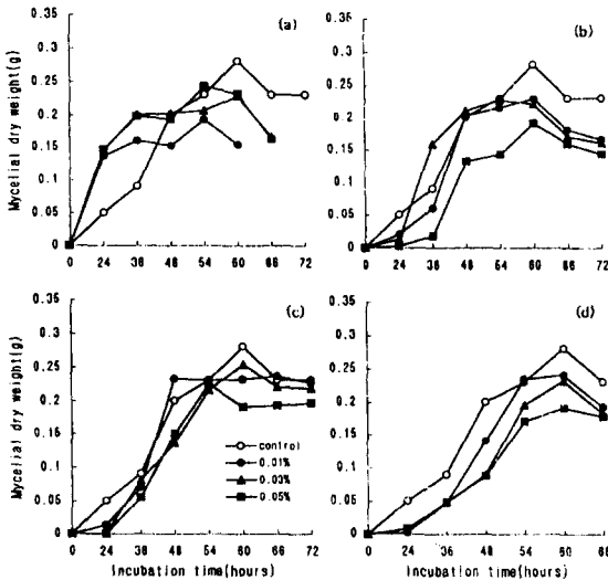
Fig. 6. The growth of A. oryzae in the presence of water (a), methanol exact (b), hexane fraction (c), and chloroform fraction (d) from A. rugosa .
