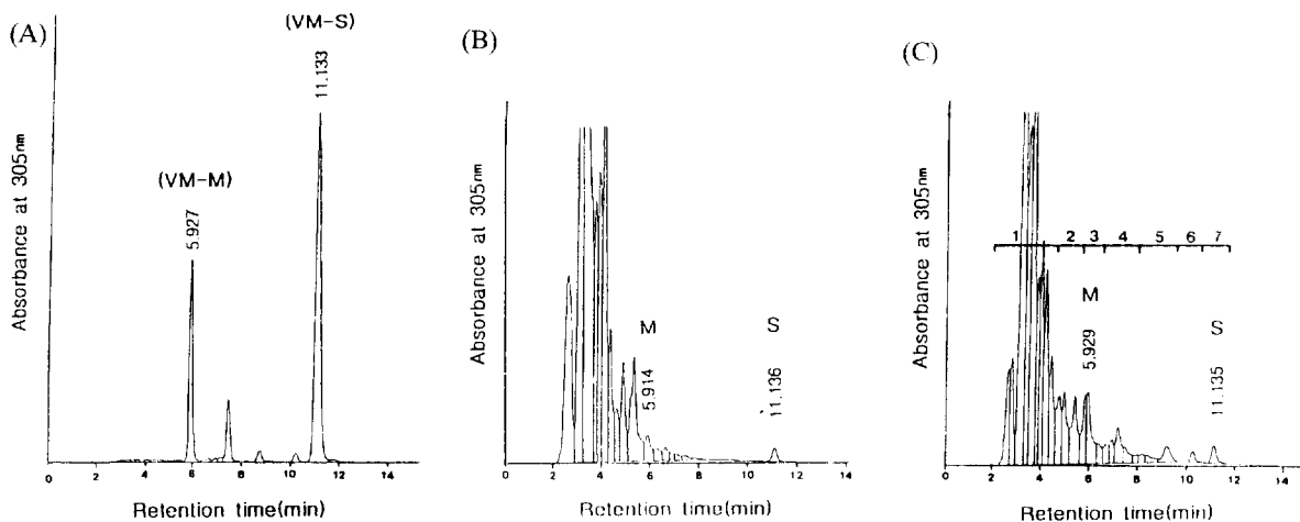
Fig. 1. HPLC chromatograms of extracts by S. graminofaciens . 300 ng/ml of synthetic VB-C was added at cultivation time of 12 hours, and culture conditions and analysis procedures were described in Materials and Methods. The elution was done on an ODS column (Shimadzu Shimpak, 4.6×300 mm) with 50% CH_3CN containing 0.1% TFA as solvent at a flow rate of 1.0 ml/min and detected at 305 nm. (A) standard virginiamycin M and S (B) - VB-C(30 hours) (C) + VB-C(30 hours).
