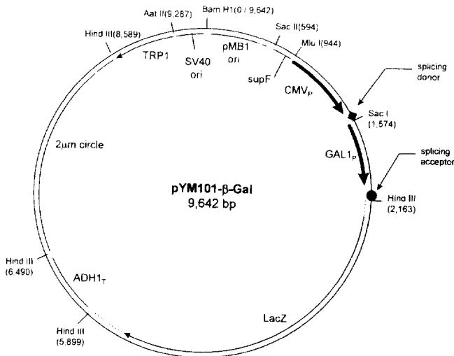
Fig. 2. Physical map of pYM101- \beta -Gal. Abbreviations used are the same as in Fig. 1.
