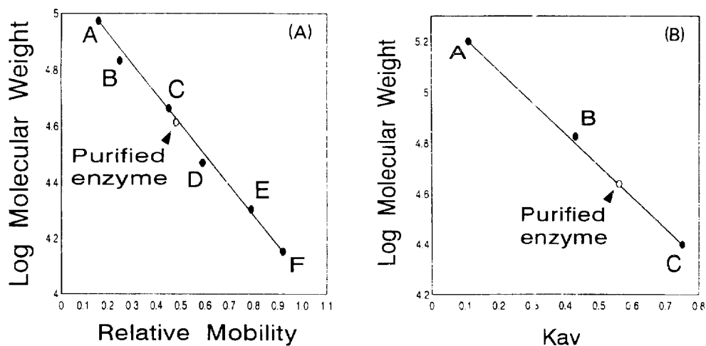
Fig. 3. Molecular weight determination of purified proteinase. (A) Molecular weight determination by SDS-PAGE. A-F are standard proteins, phosphorylase b (94,000), bovine serum albumin (67,000), ovalbumin (43,000), carbonic anhydrase (30,000), trypsin inhibitor (20,100) and \alpha -lactalbumin (14,400), respectively. (B) Molecular weight determination by Sephacryl S-200 HR molecular sieve chromatography. A-C are standard proteins, aldolase (158,000), bovine serum albumin (67,000) and chymotrypsinogen A (25,000), respectively.
