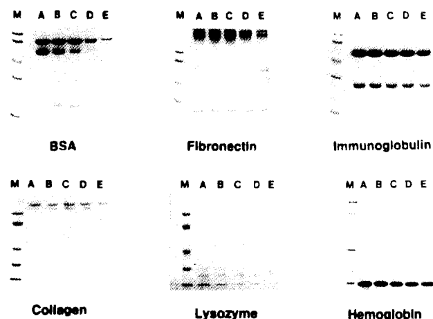
Fig. 5. Substrate specificity of purified proteinase. Each reaction mixture containing proteinase was run under the condition described in materials and methods. Lane A-E, each substrate was incubated with proteinase for 0, 2, 4, 6 and 12 h at 37°C, respectively. Lane M, standard marker proteins.
