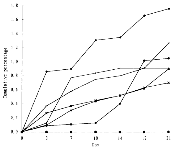
Fig. 4. Evolution of radioactive volatile compounds from phenanthrene during biodegradation by white-rot fungi. -▲-: Phanerochaete chrysosporium , -●-: Pleurotus ostreatus , -◆-: Coriolus versicolor KR-11W, -×-: Coriolus versicolor KR-65W, -+-: Irpex lacteus , -+-: Microporus vernicipes , -■-: Control.
