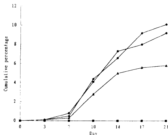
Fig. 5. Evolution of radioactive carbon dioxide from pyrene biodegradation by white-rot fungi. -■-: Control, -▲-: Phanerochaete chrysosporium , -●-: Coriolus versicolor KR-11W, -◆-: Irpex lacteus .
